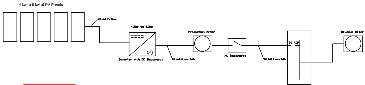
4.2 to 5.0 KW PV System Layout
